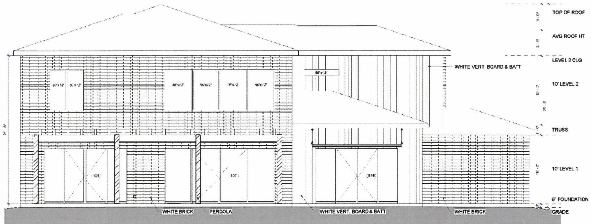
REAR ELEVATION SCALE 1/2" = 1'-0"
