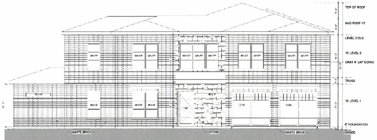
FRONT ELEVATION SCALE 1/2" = 1'-0"
