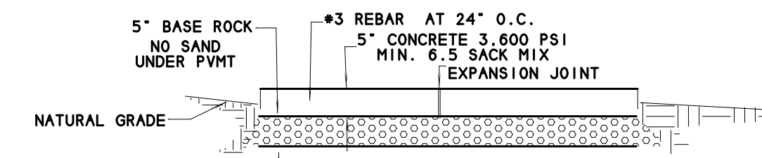
CONCRETE PAVEMENT CROSS SECTION
