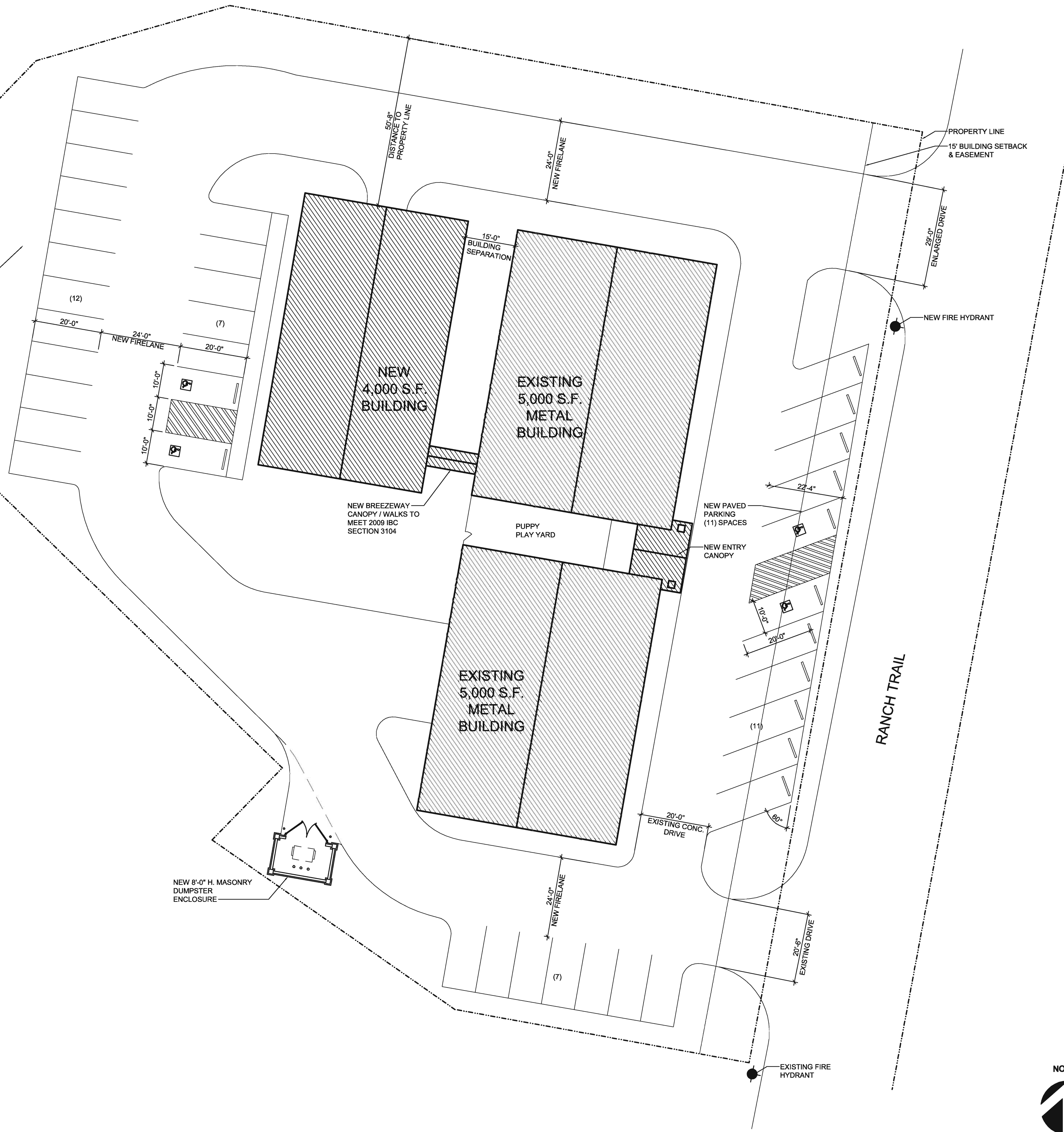
SITE PLAN SCALE: 1/16" = 1'-0"
