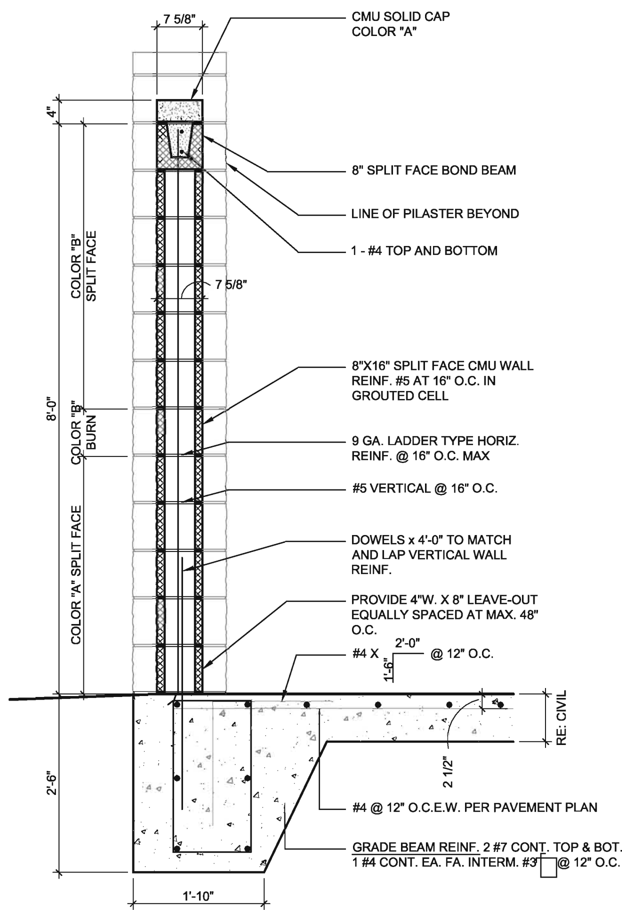
DUMPSTER ENCLOSURE SECT. 2 SCALE: 3/4" = 1'-0"
