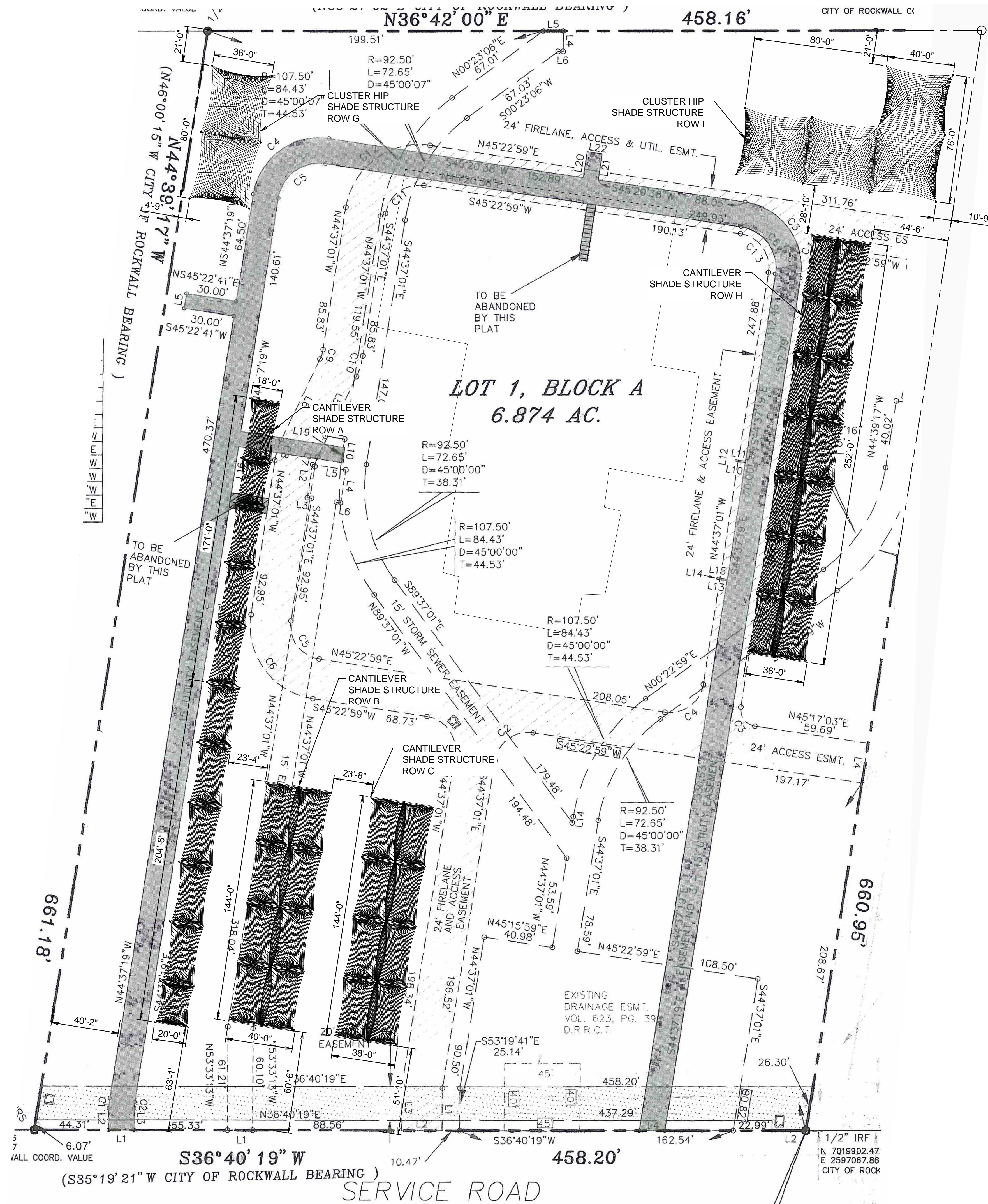
SITE PLAN SCALE: 1/32" = 1'-0"
