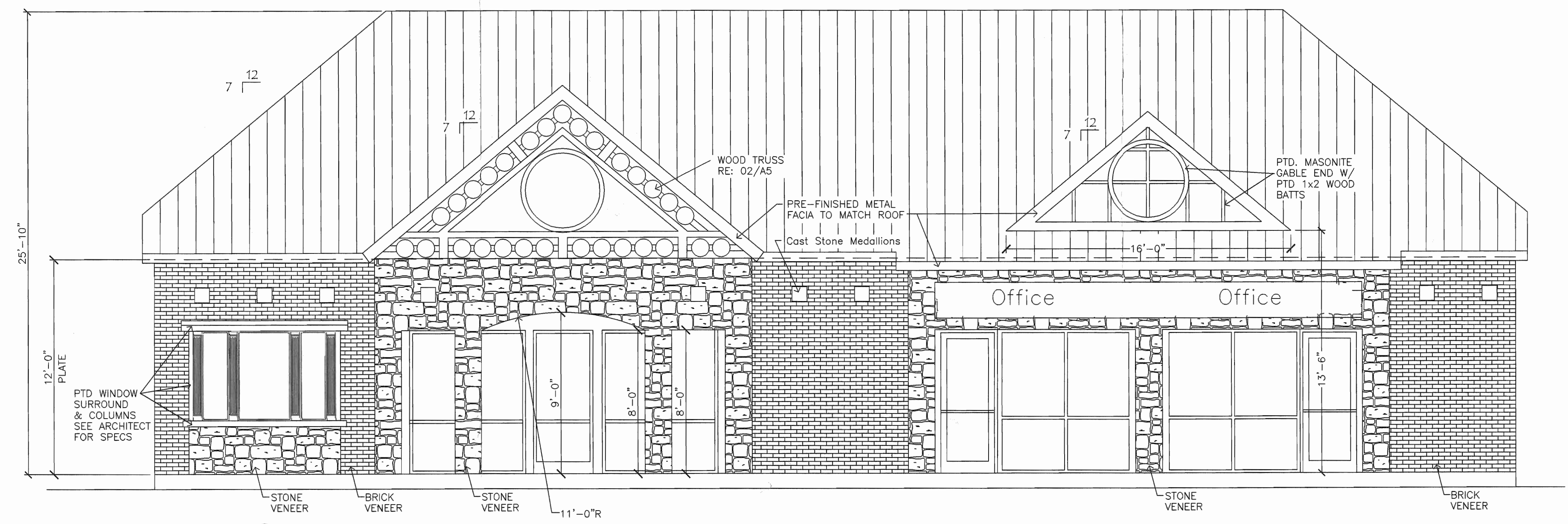
01 FRONT ELEVATION SCALE: 1/4" = 1'-0"
