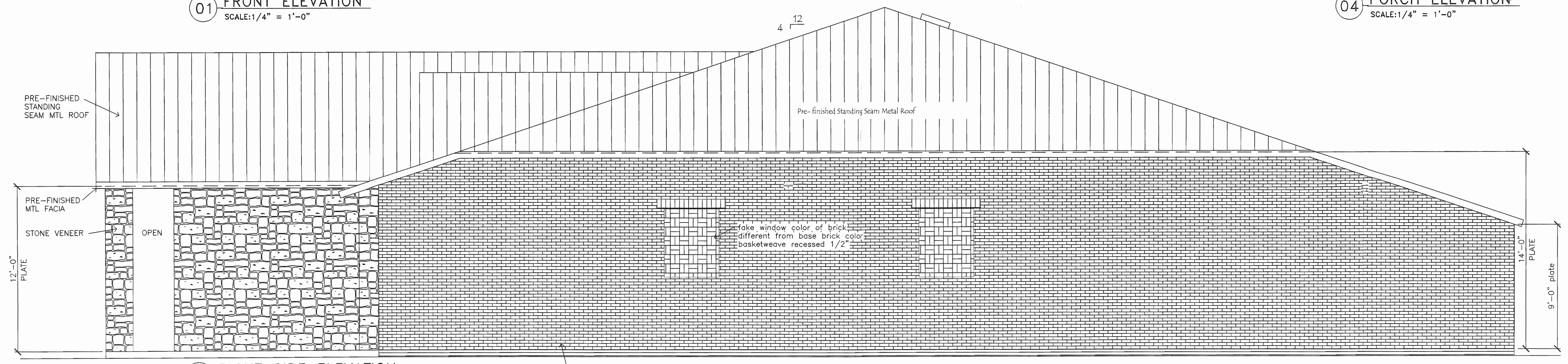
02 RIGHT SIDE ELEVATION SCALE: 1/4" = 1'-0"
