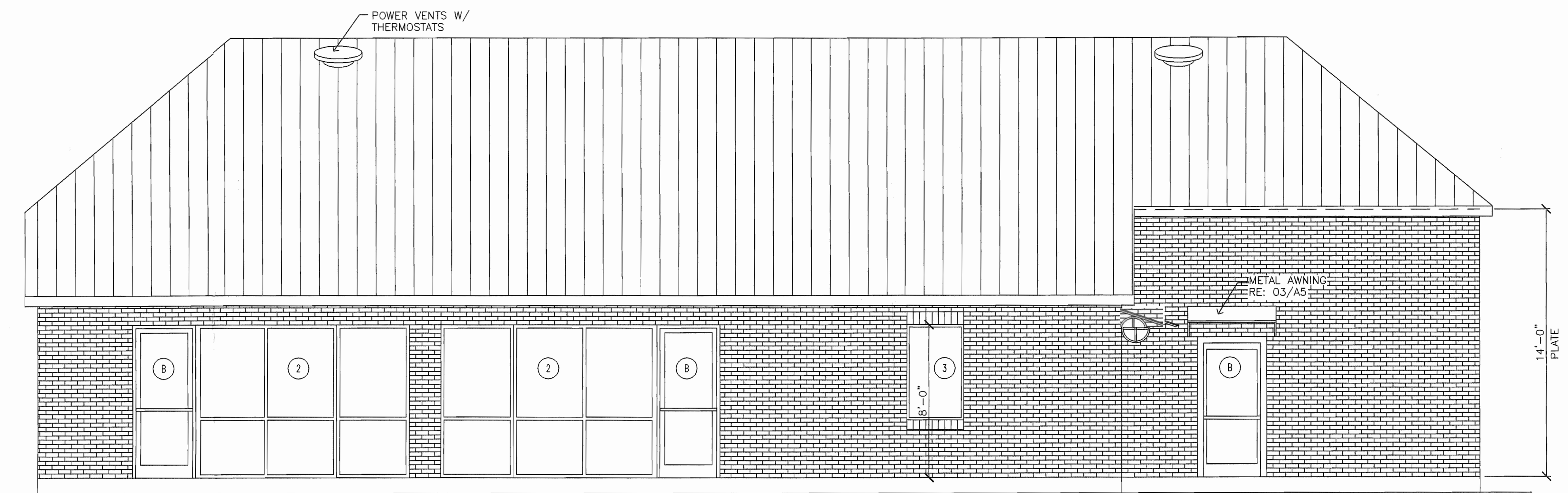
03 REAR ELEVATION SCALE: 1/4" = 1'-0"
