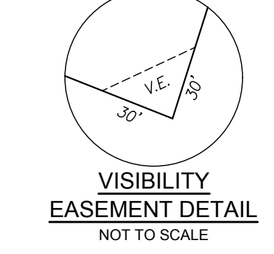
VISIBILITY EASEMENT DETAIL NOT TO SCALE
