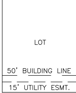
TYPICAL LOT DETAIL
