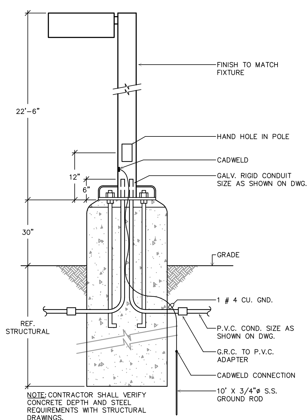
02 TYPES 'AA' & 'AB' MOUNTING DETAIL SCALE: NOT TO SCALE
