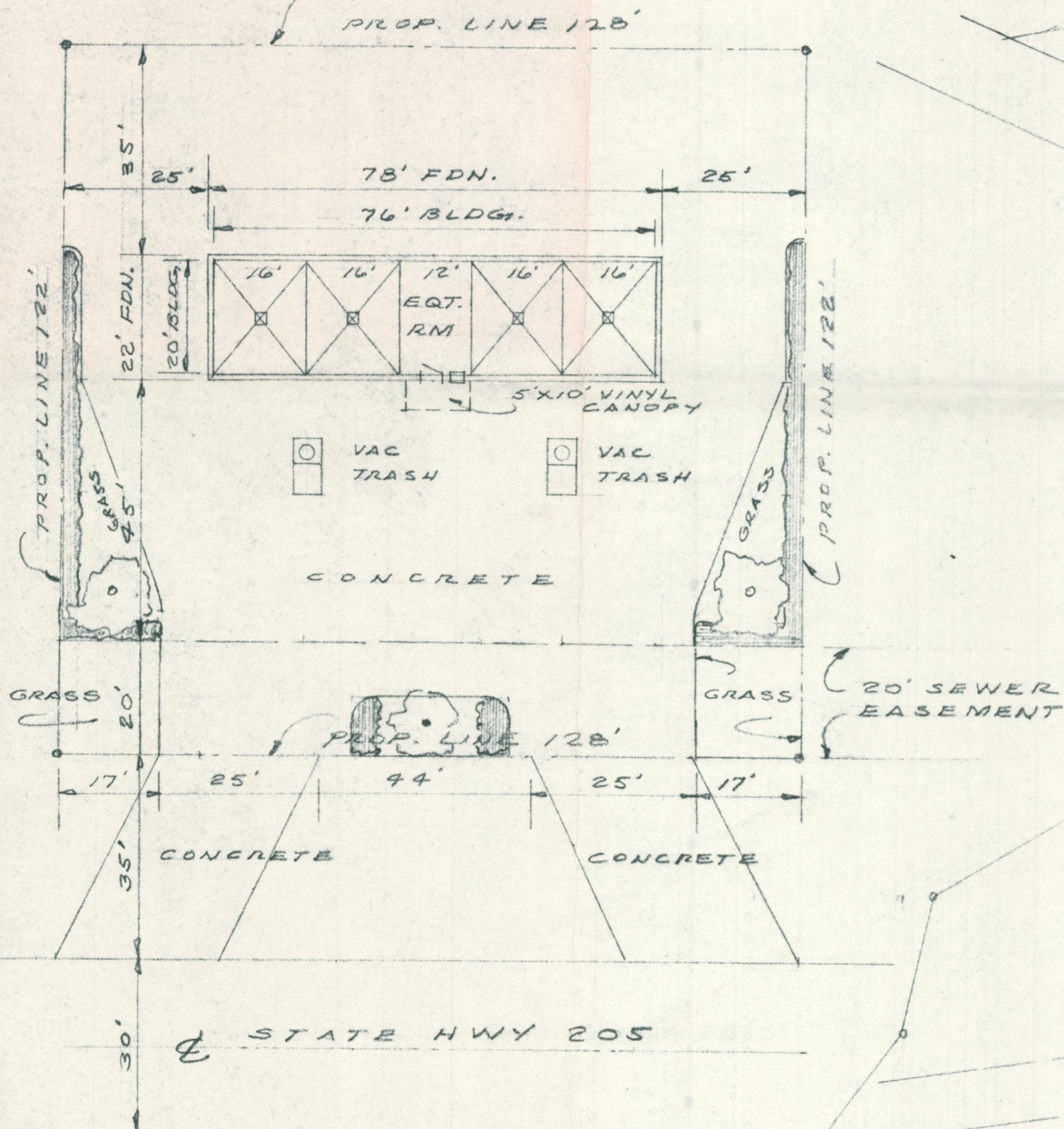
PLOT PLAN SCALE 1"=20'
