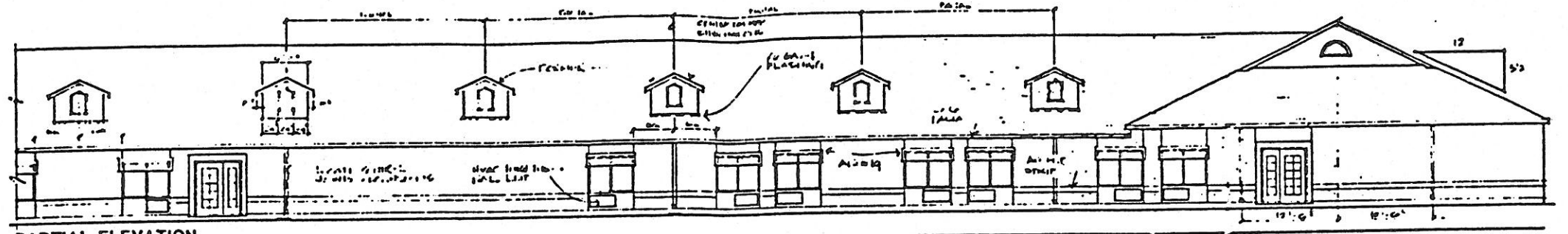
PARTIAL ELEVATION 1/8" = 1'-0"
