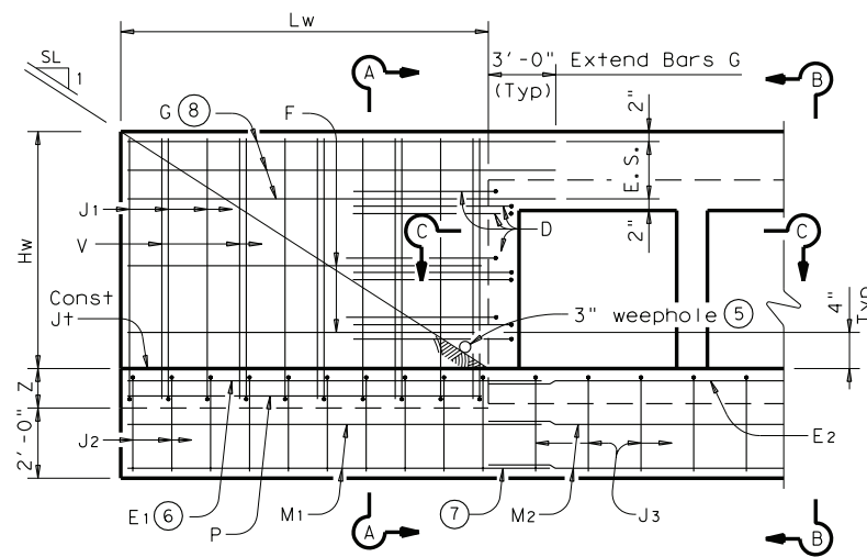
PARTIAL ELEVATION
