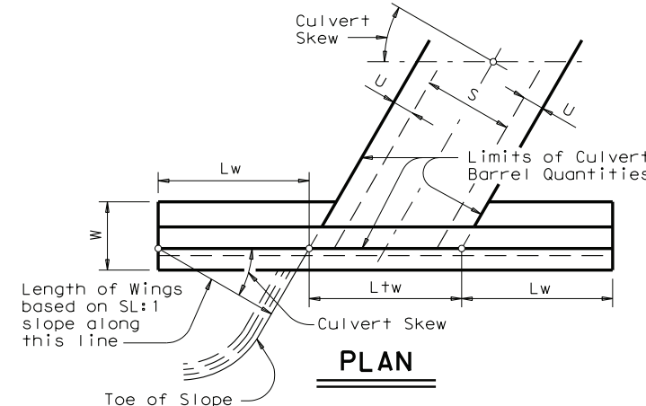
DETAILS FOR SKEWED BOX CULVERTS
