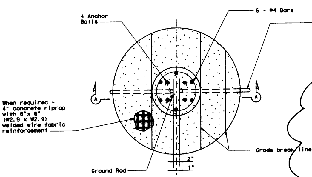
FOUNDATION DETAIL
