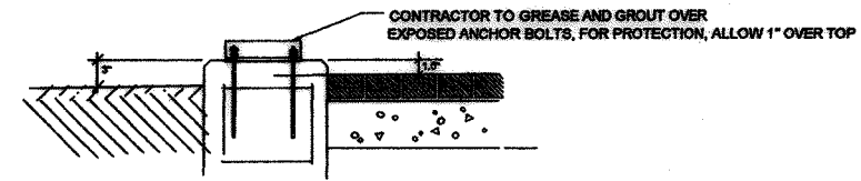
SECTION GROUT CAP
