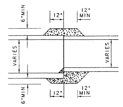
CONCRETE COLLAR FOR PIPE CONNECTION
