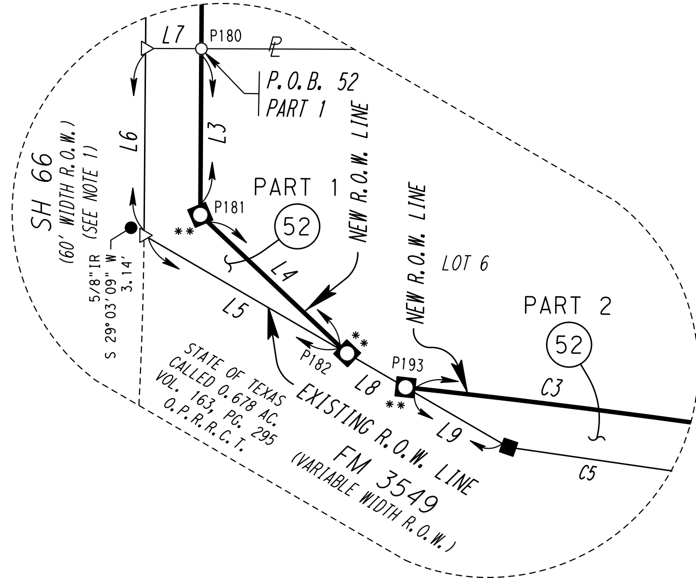
PARCEL 52 PART 1 & 2 DETAIL 1"=20' FULL SCALE 1"=40' HALF SCALE
