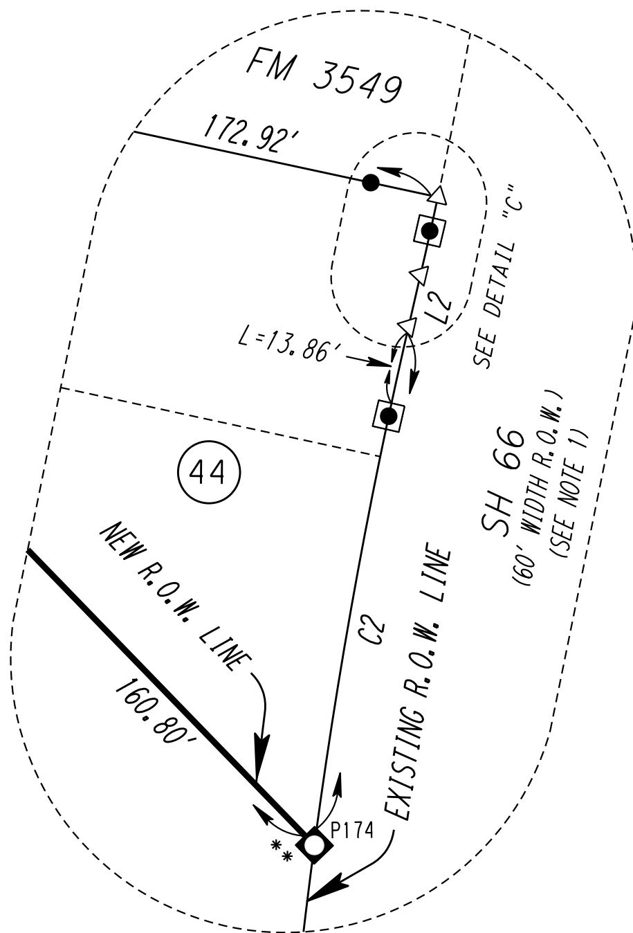
PARCEL 44 DETAIL 1"=20' FULL SCALE 1"=40' HALF SCALE
