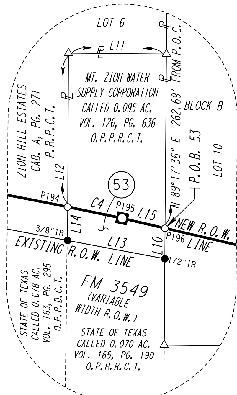
PARCEL 53 DETAIL 1"=20' FULL SCALE 1"=40' HALF SCALE
