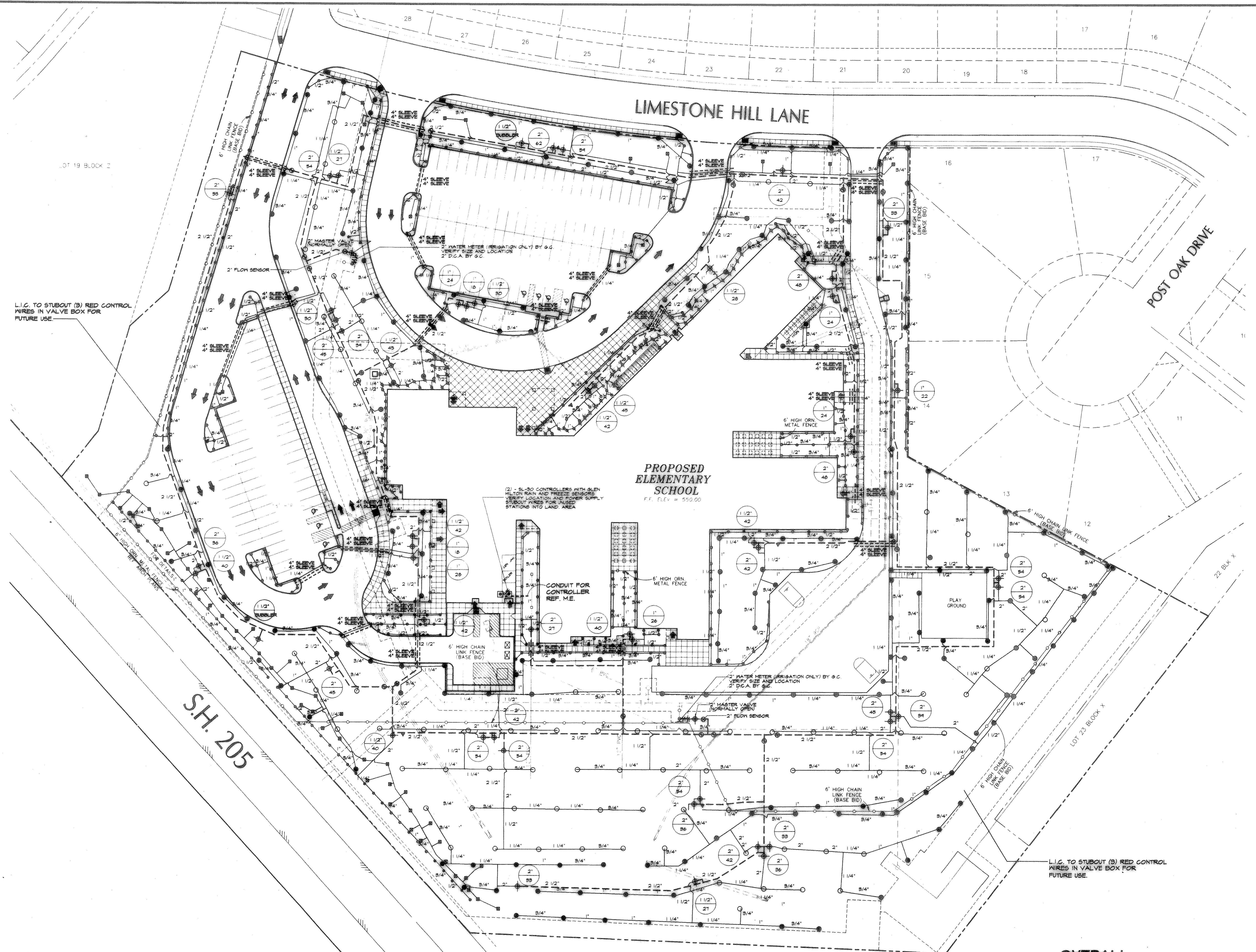
OVERALL IRRIGATION PLAN SCALE: 1"=40'-0"
