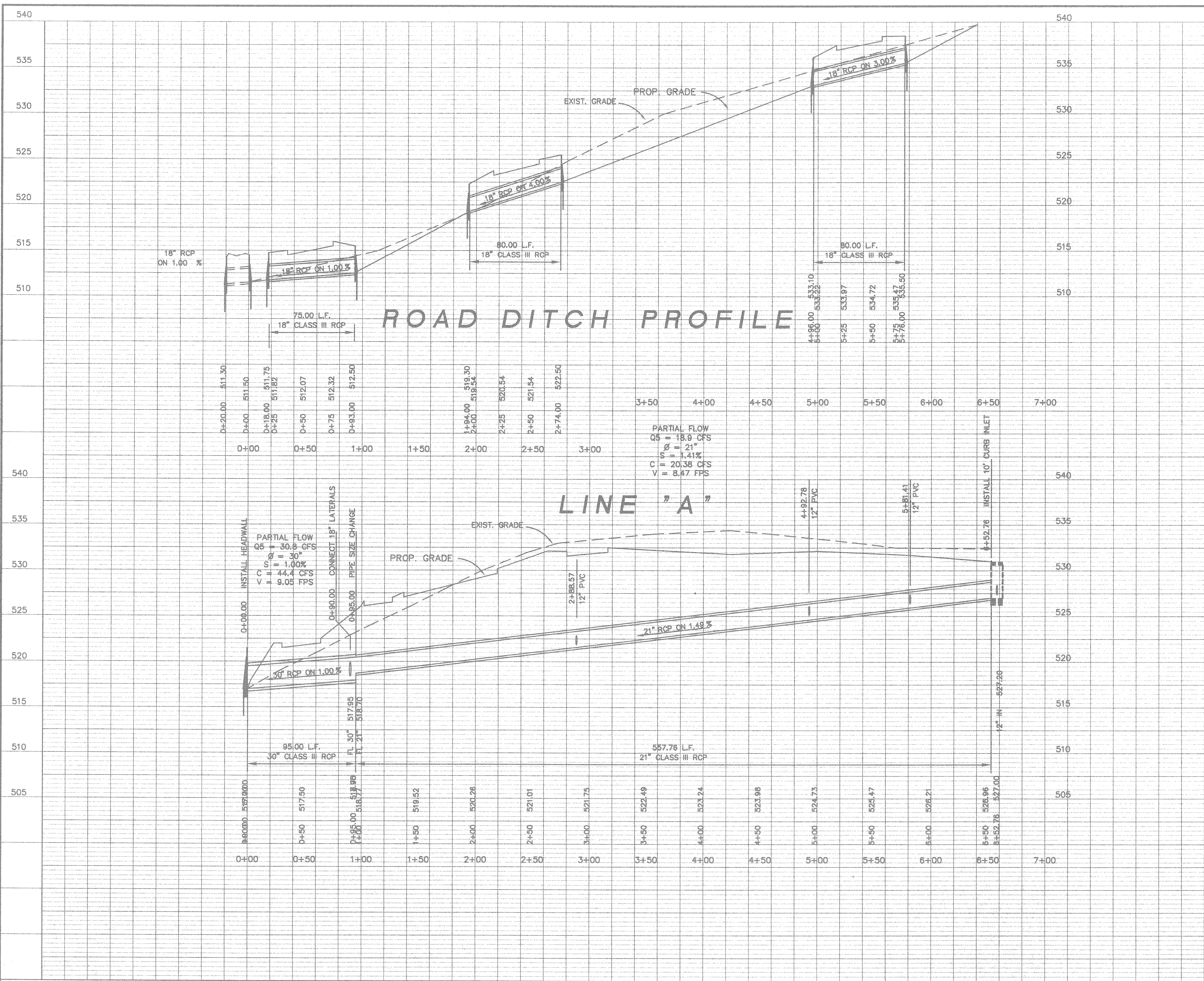
STORM SEWER PROFILE Scale 1"=40' H 1"=5' V
