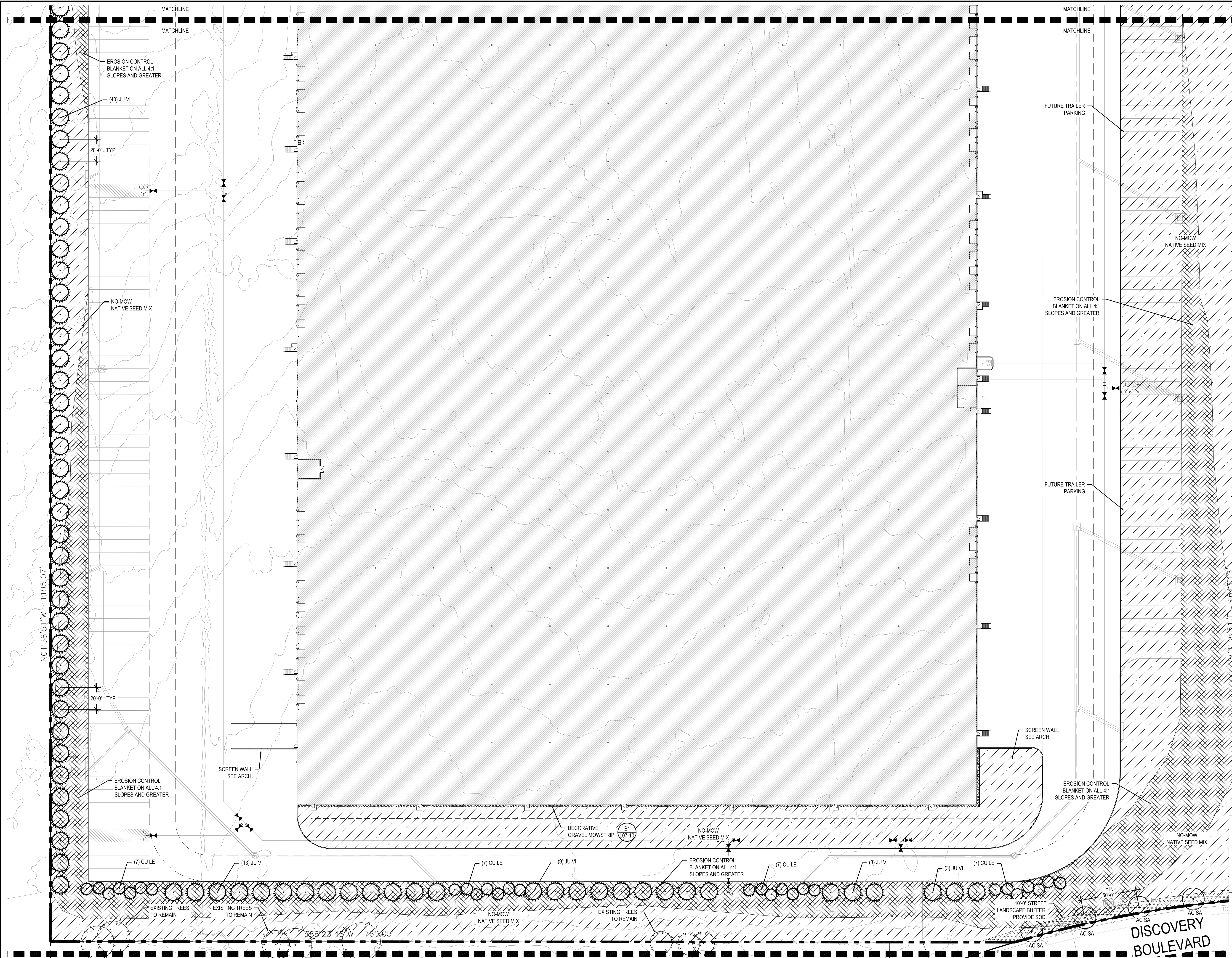
1 LANDSCAPE PLAN - AREA 2 SCALE: 1" = 40'-0"
