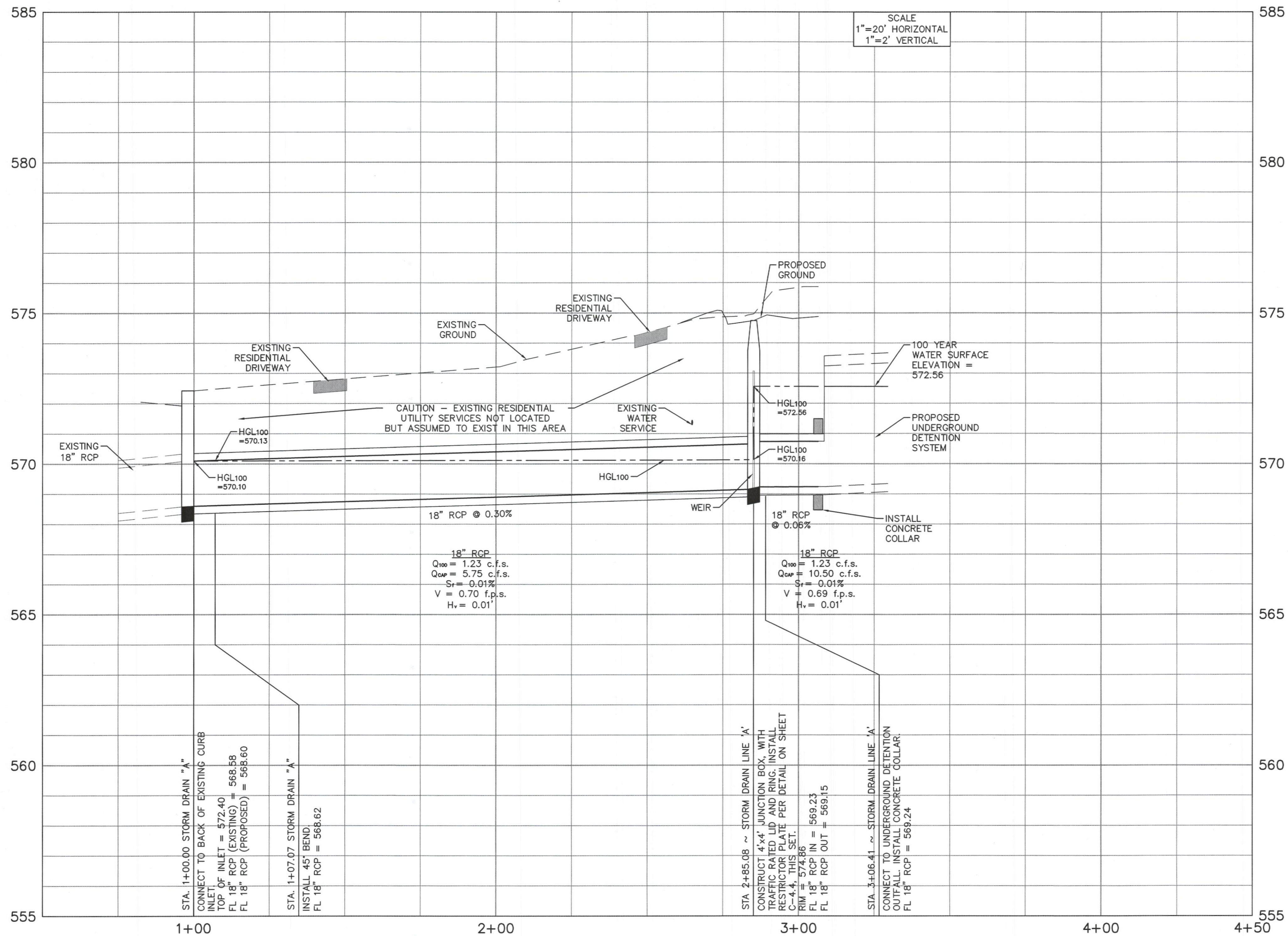
STORM DRAIN LINE "A"
