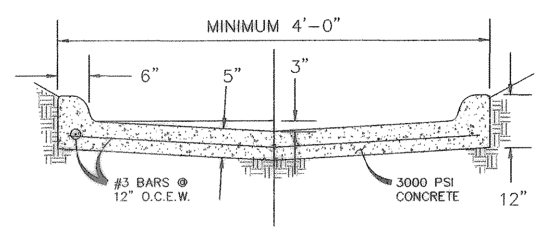
CURBED OVERFLOW FLUME INSTALL JIGGIE BAR @ 50' INTERVALS
