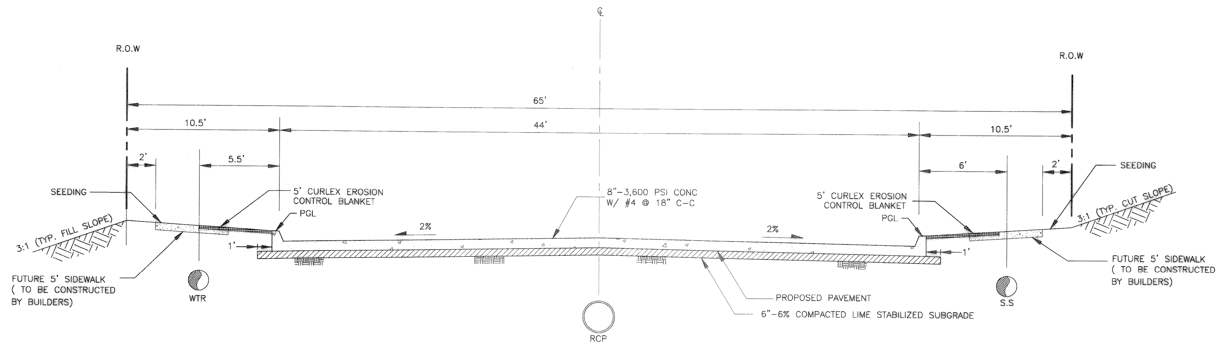
TYPICAL PAVING SECTION & UTILITY LOCATIONS FOR MEDICAL DRIVE
