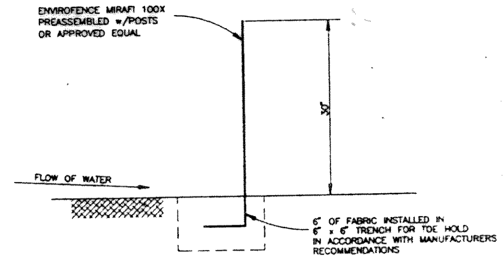
SILTATION FENCE EROSION CONTROL DEVICE
