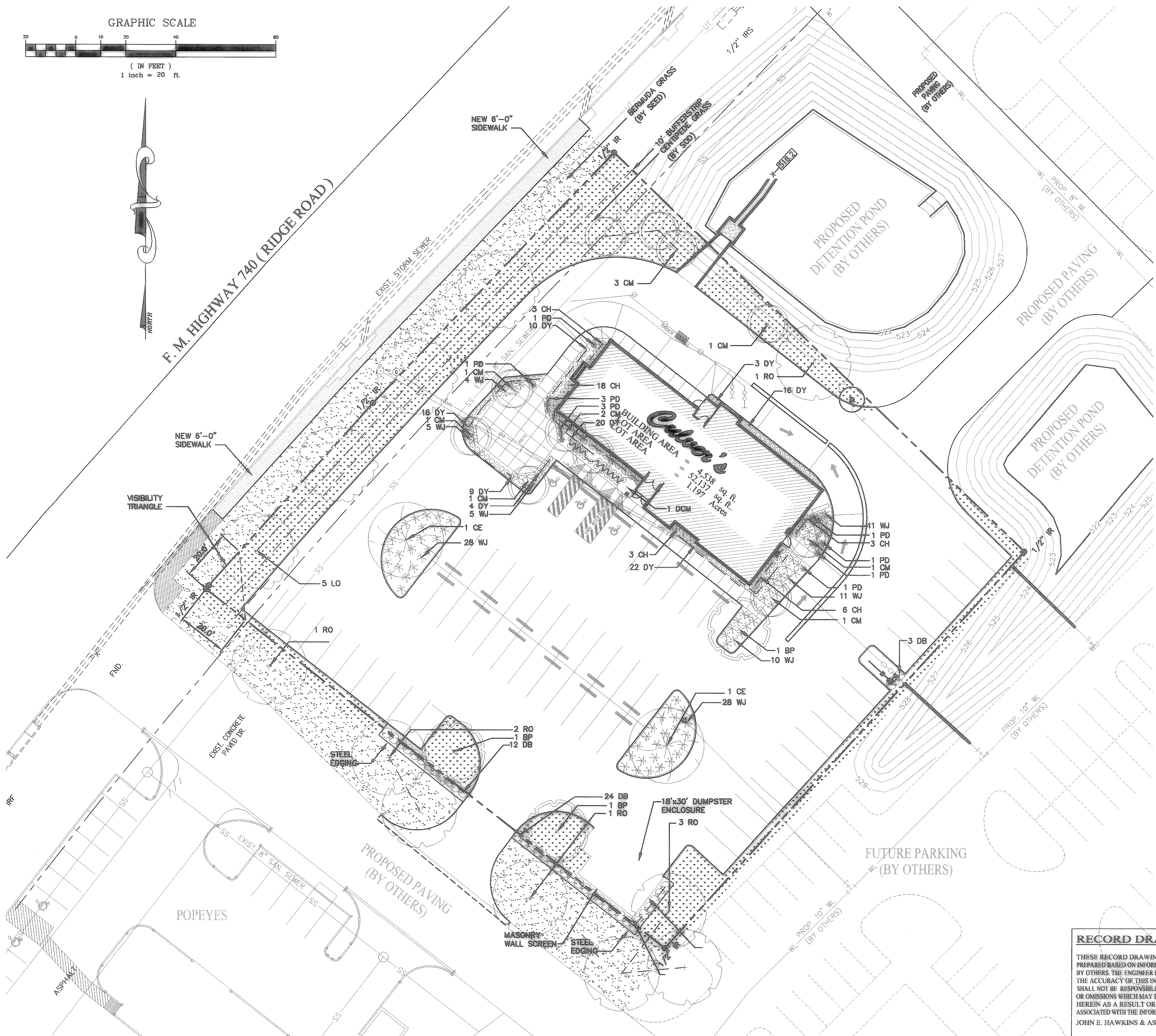
LANDSCAPE PLAN SCALE: 1"= 20'
