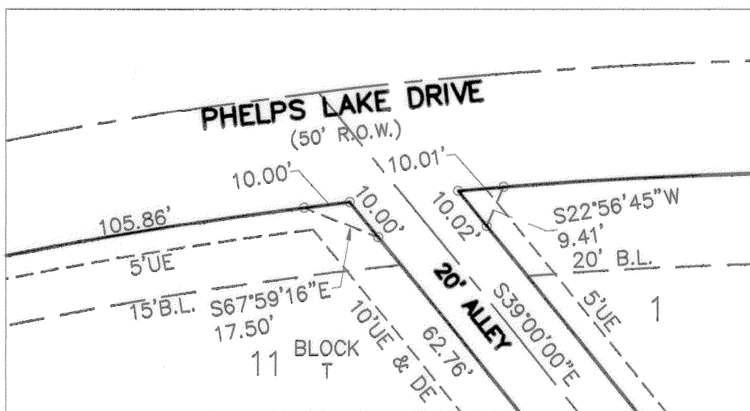
CORNER CLIP DETAILS
