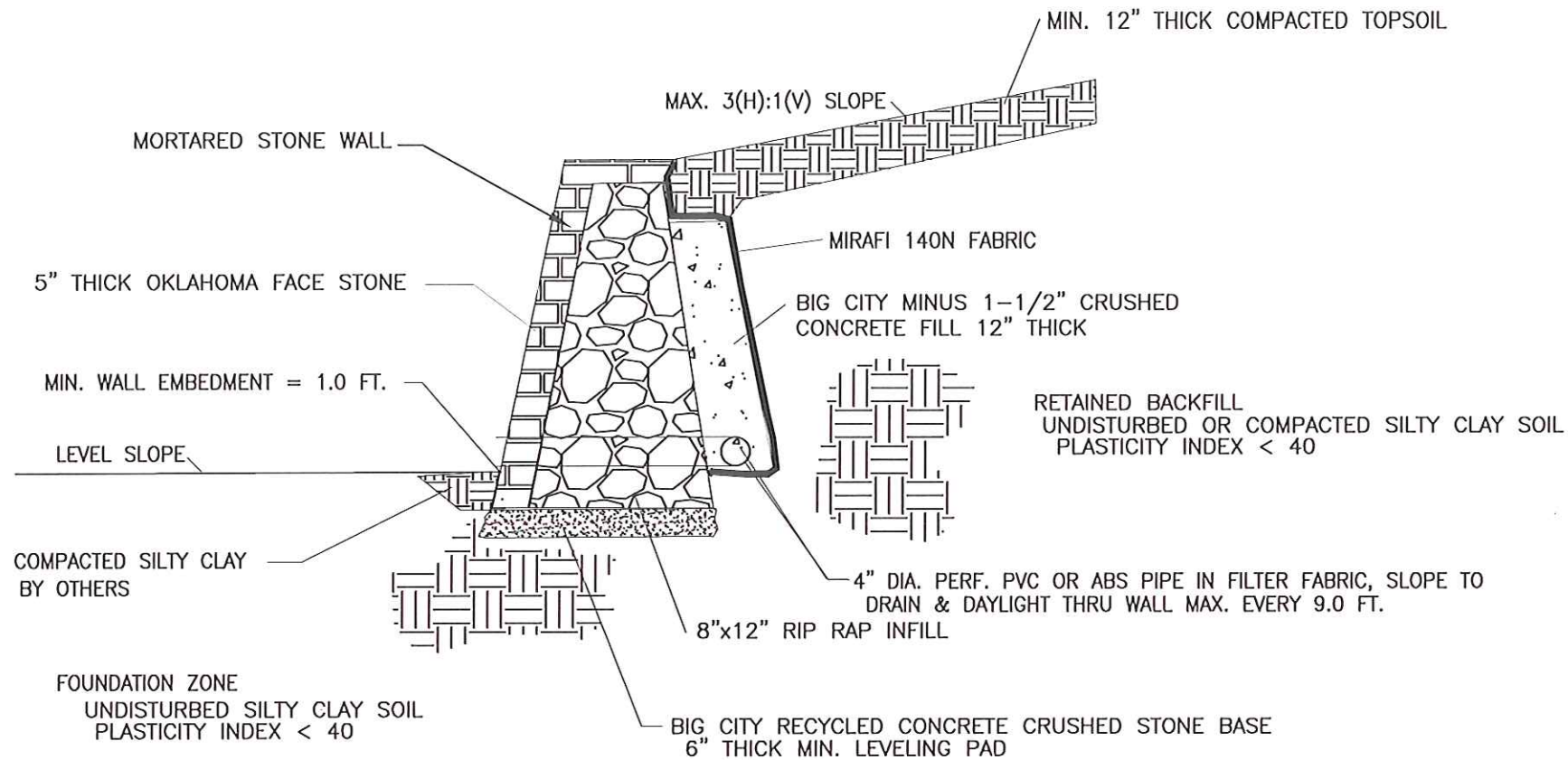
TYPICAL MORTARED WALL DIMENSIONS SCALE: NONE
