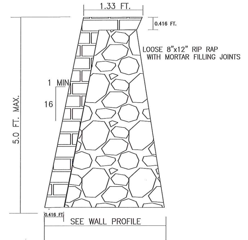
TYPICAL MORTARED WALL DIMENSIONS SCALE: NONE
