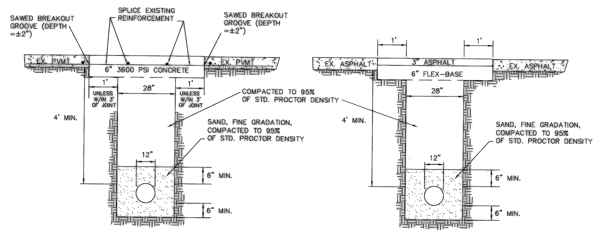
UTILITY EXCAVATION & EMBEDMENT DETAIL N.T.S.
