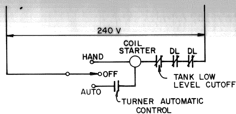
BOOSTER PUMP CONTROL SCHEMATIC
