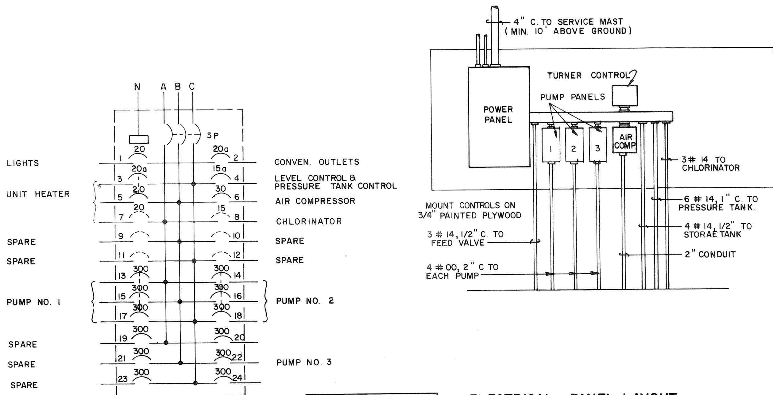
ELECTRICAL PANEL LAYOUT
