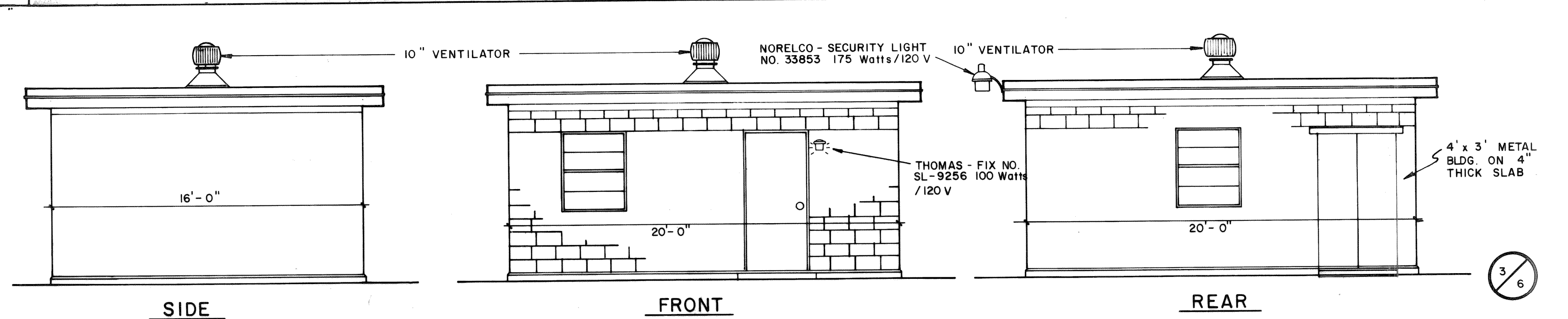
PUMP HOUSE ELEVATIONS
