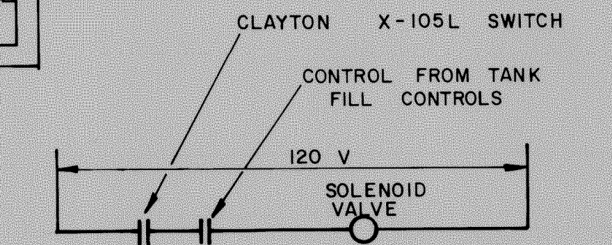
CHLORINE CONTROL SCHEMATIC
