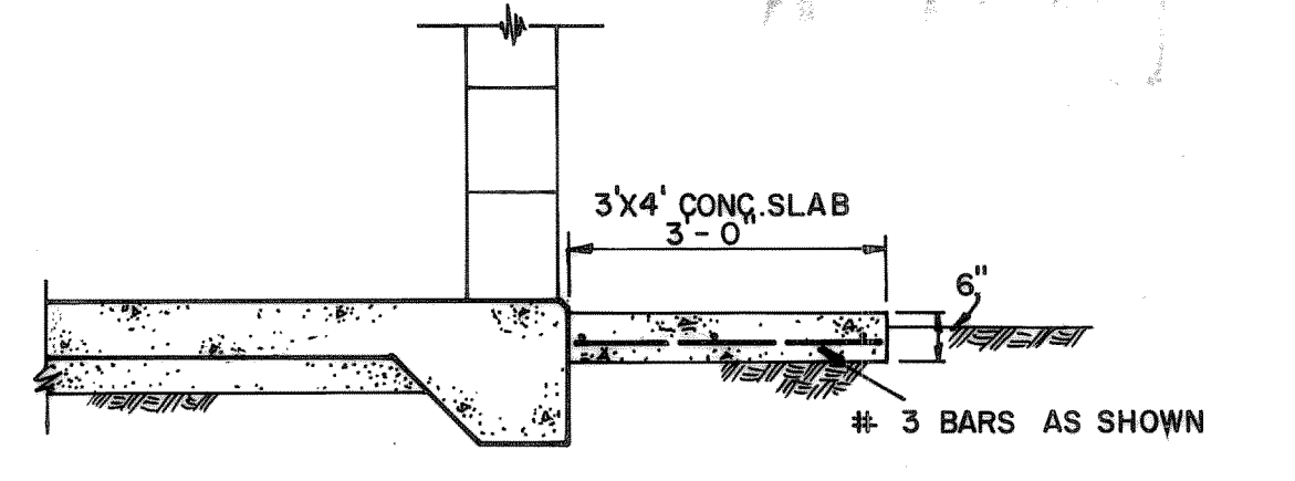
CONCRETE LANDING DETAIL SCALE: 1/2" = 1'-0"
