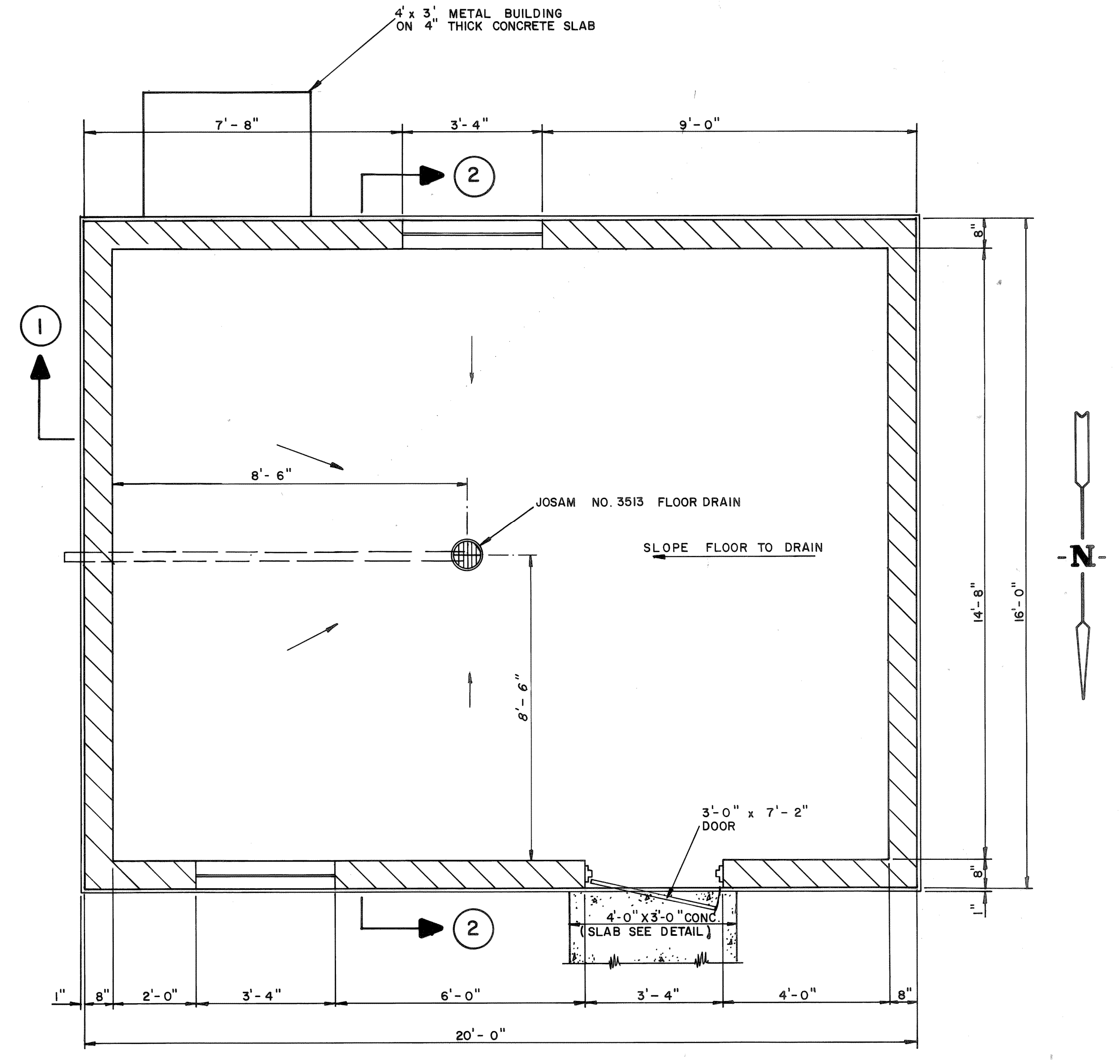
PUMP HOUSE PLAN SCALE: 1/2" = 1'-0"
