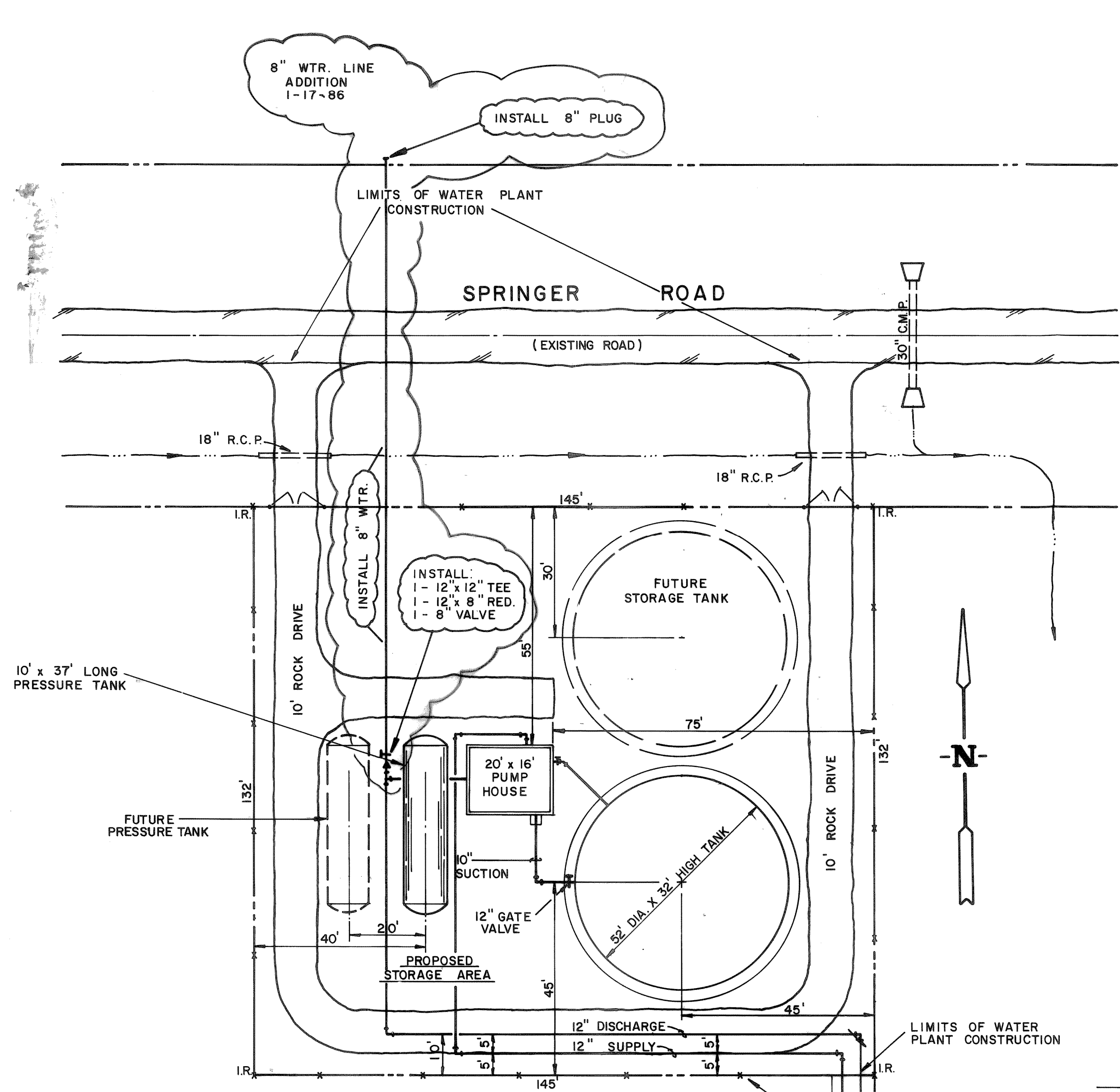
PLANT SITE SCALE: 1" = 20'
