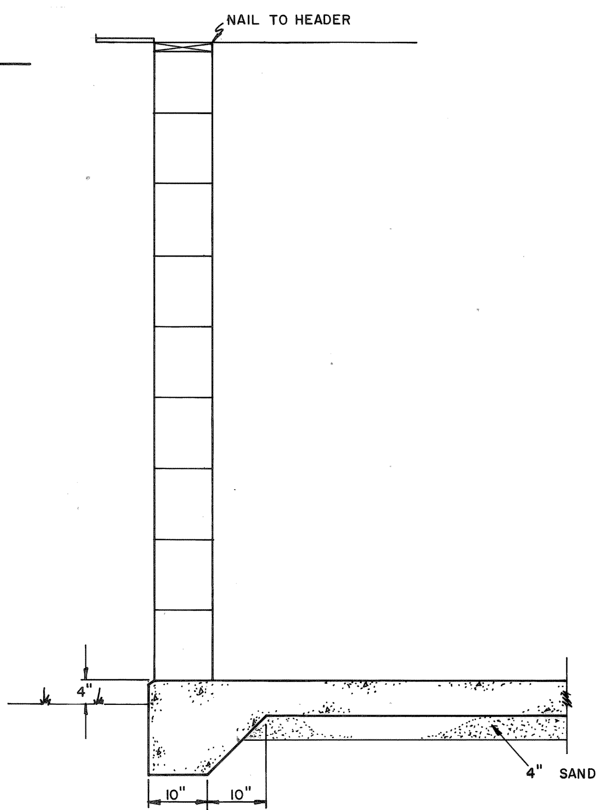
WALL SECTION 1 SCALE: 3/4" = 1'-0"
