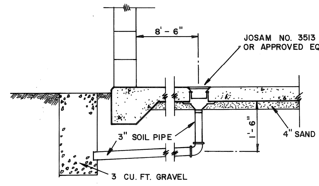
DRAIN DETAIL SCALE: 1/2" = 1'-0"
