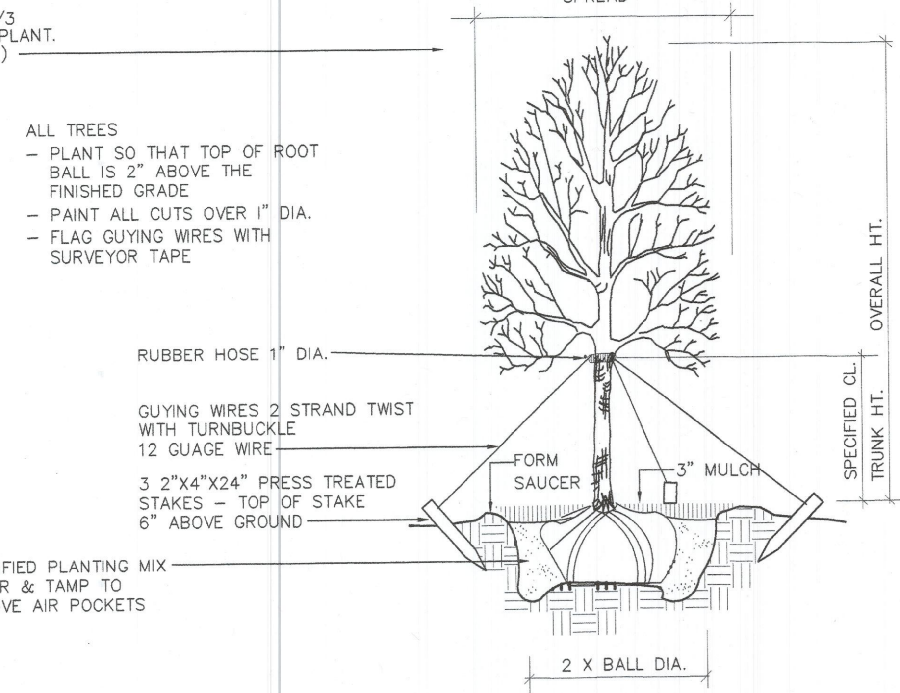
TREE PLANTING - GUY WIRES OVER 2" CALIPER
