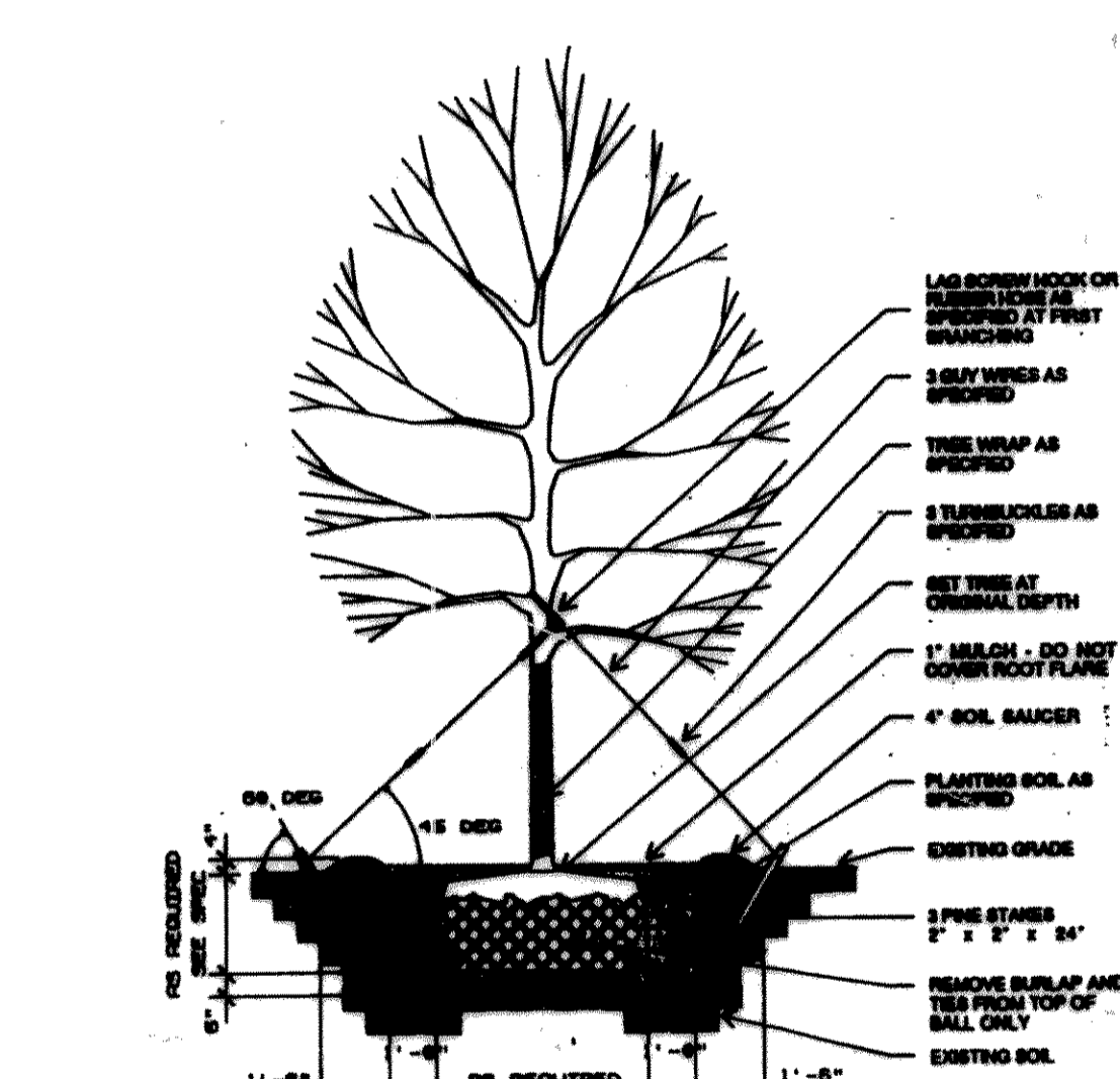
A Tree Planting Section
