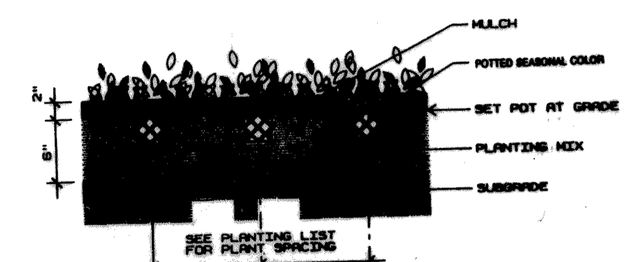
D Seasonal Color Planting Section Groundcover Planting Section
