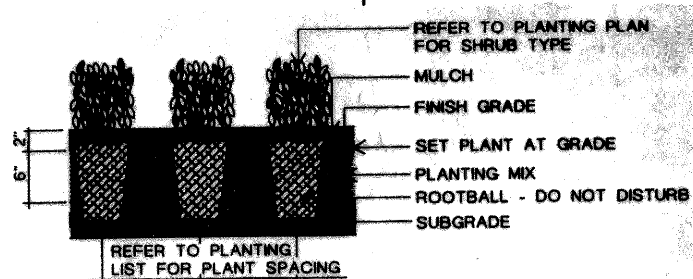
Shrub Planting Section
